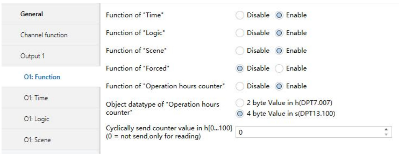
Fig. 4.11 Parameter window "Ox: Operation hours counter"
