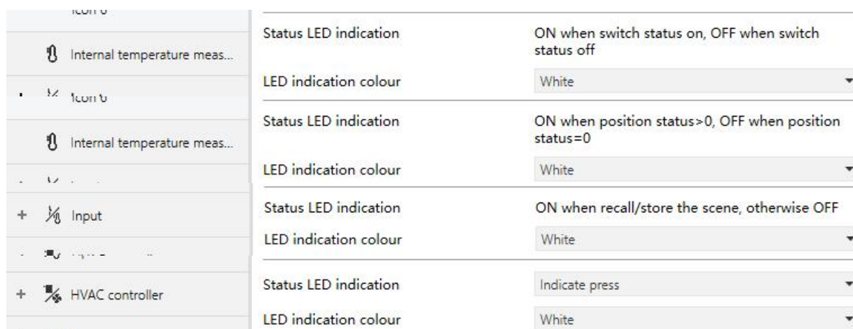
Fig.5.6.2.6 Parameter setting of LED indication function
