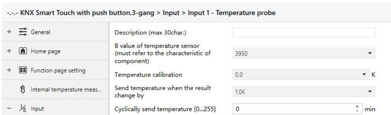
Fig.5.3.1 Parameter setting of temperature probe
